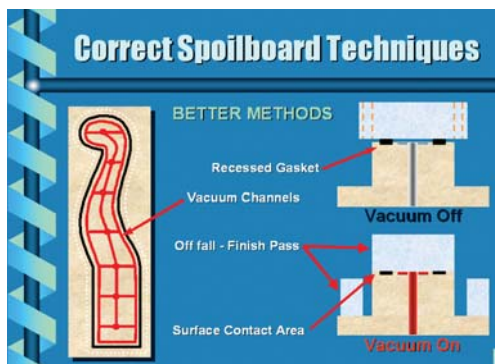
Figure 1. Correct spoilboard techniques.
